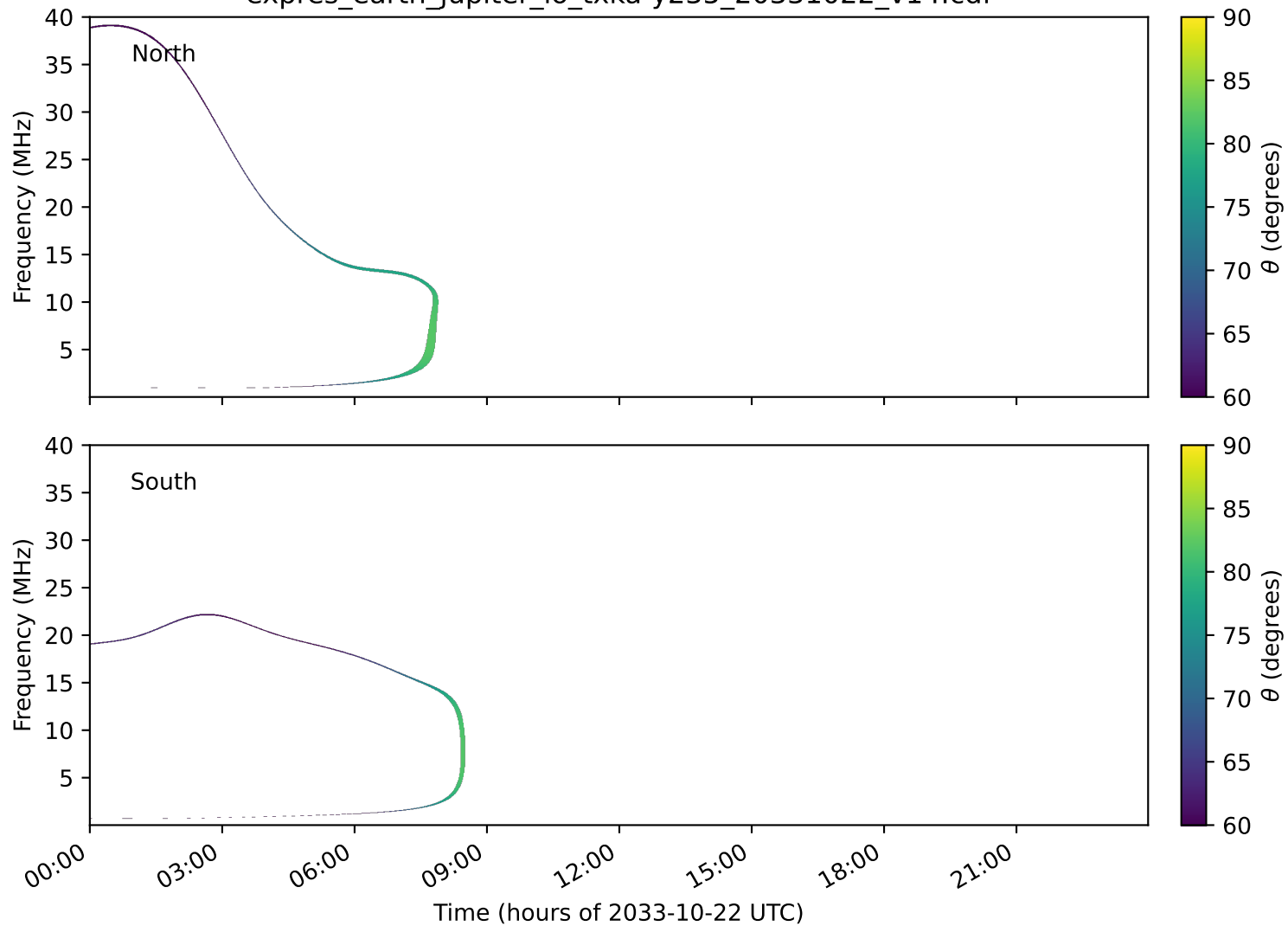
expres_earth_jupiter_io_txka-y235_20331022_v14.cdf
