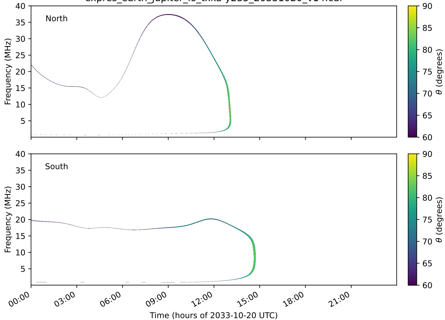
expres_earth_jupiter_io_txka-y235_20331020_v14.cdf
