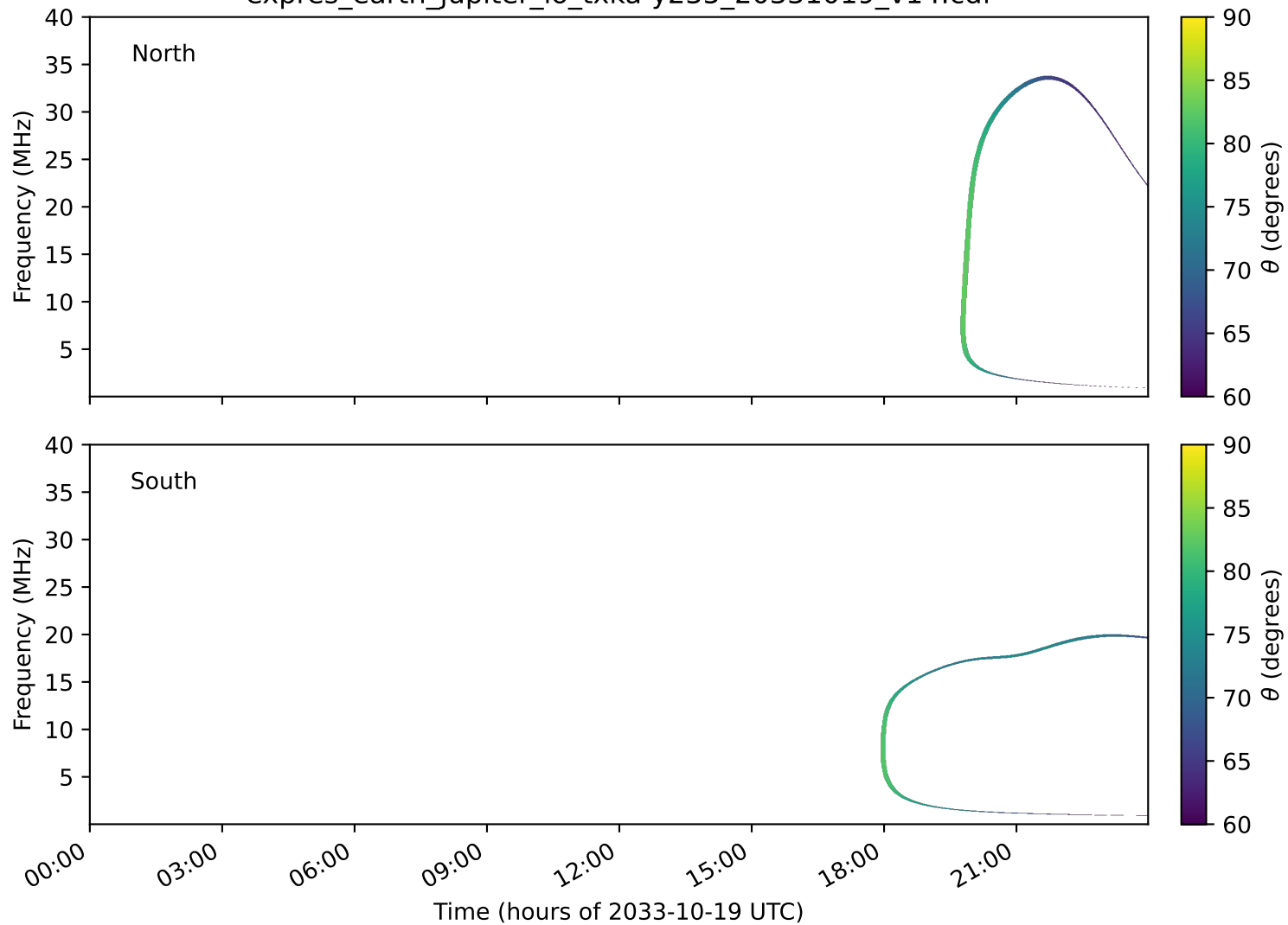
expres_earth_jupiter_io_txka-y235_20331019_v14.cdf
