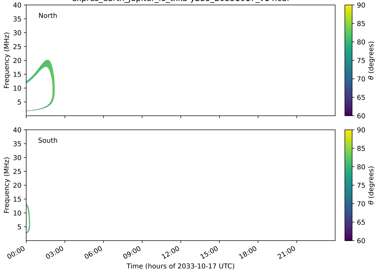
expres_earth_jupiter_io_txka-y235_20331017_v14.cdf
