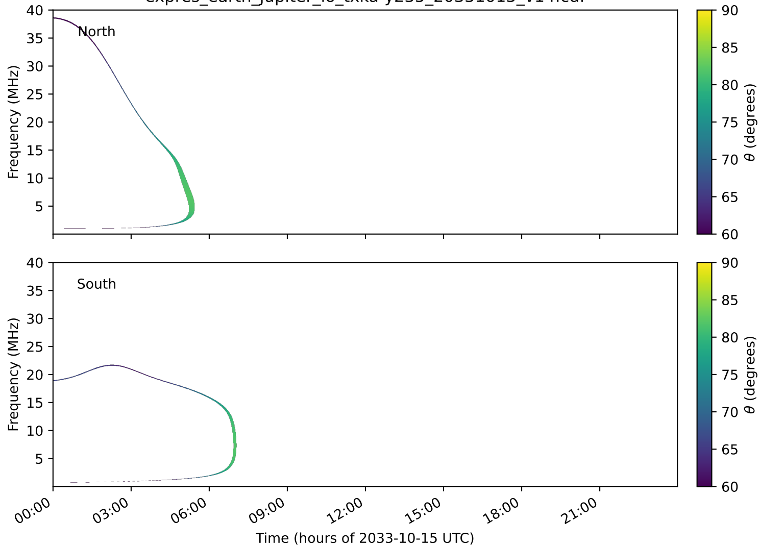
expres_earth_jupiter_io_txka-y235_20331015_v14.cdf
