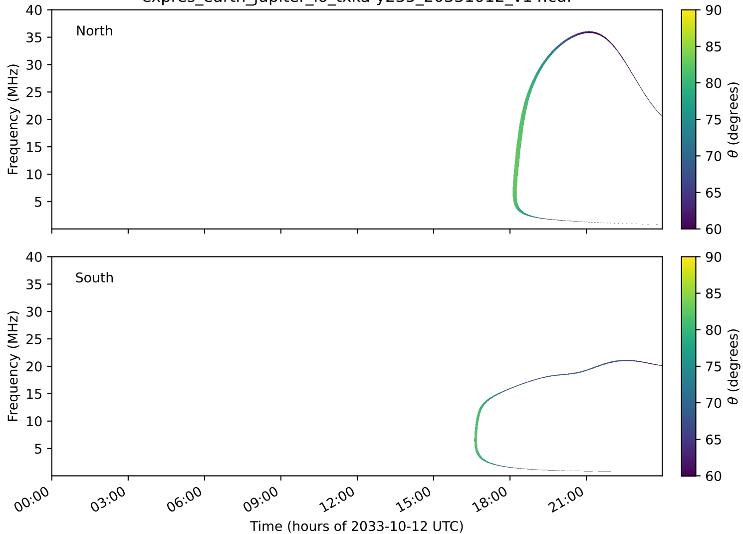
expres_earth_jupiter_io_txka-y235_20331012_v14.cdf
