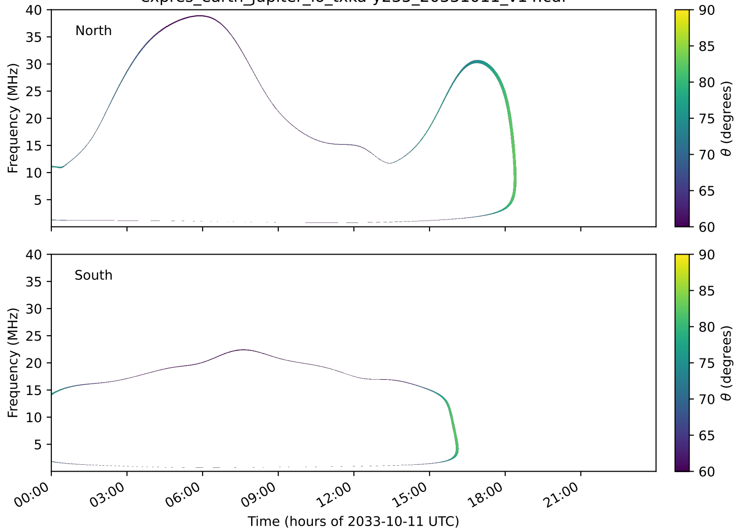
expres_earth_jupiter_io_txka-y235_20331011_v14.cdf
