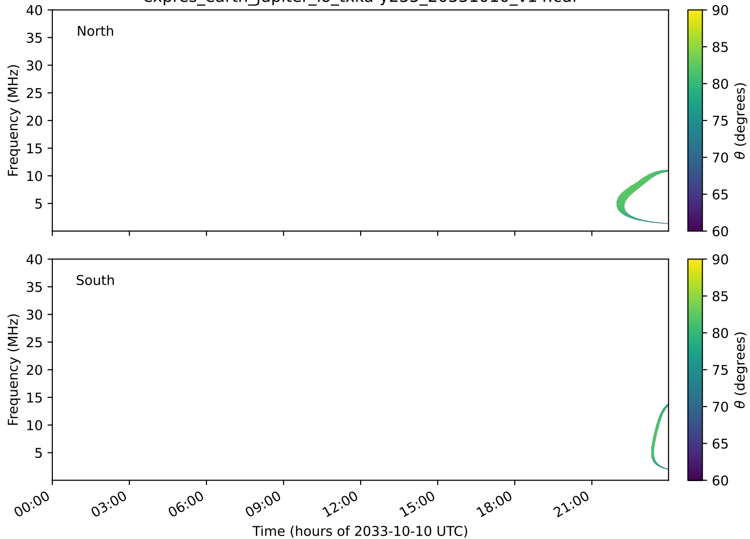
expres_earth_jupiter_io_txka-y235_20331010_v14.cdf
