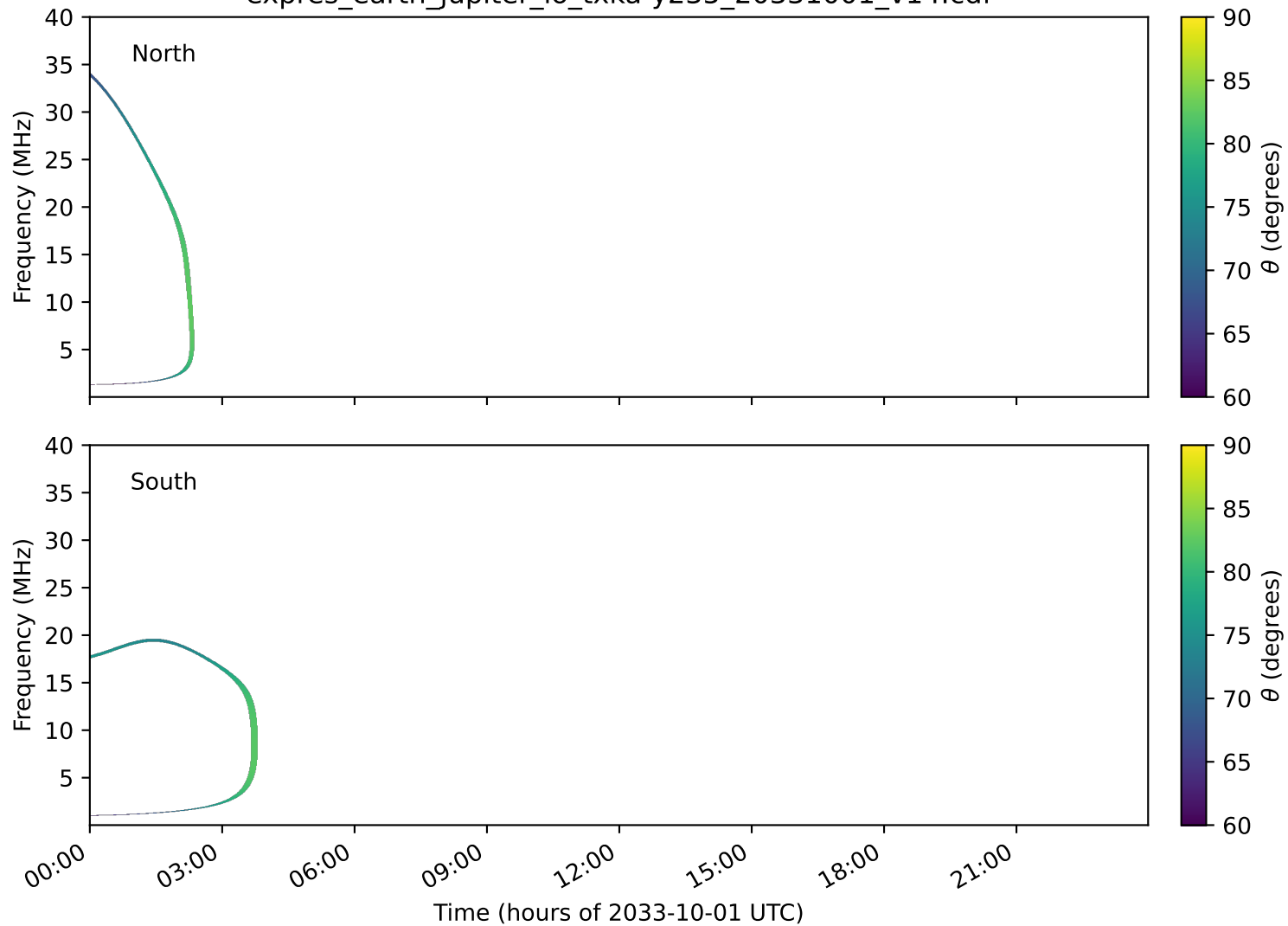
expres_earth_jupiter_io_txka-y235_20331001_v14.cdf
