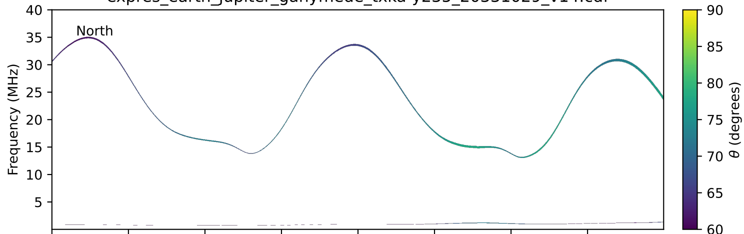
expres_earth_jupiter_ganymede_txka-y235_20331029_v14.cdf
