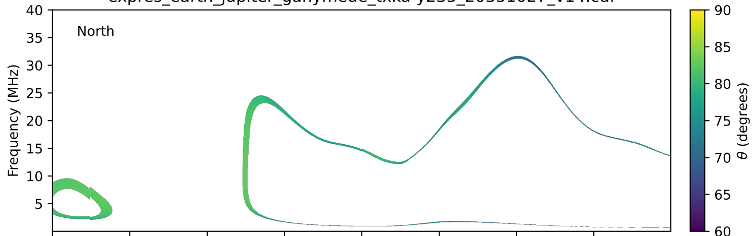
expres_earth_jupiter_ganymede_txka-y235_20331027_v14.cdf
