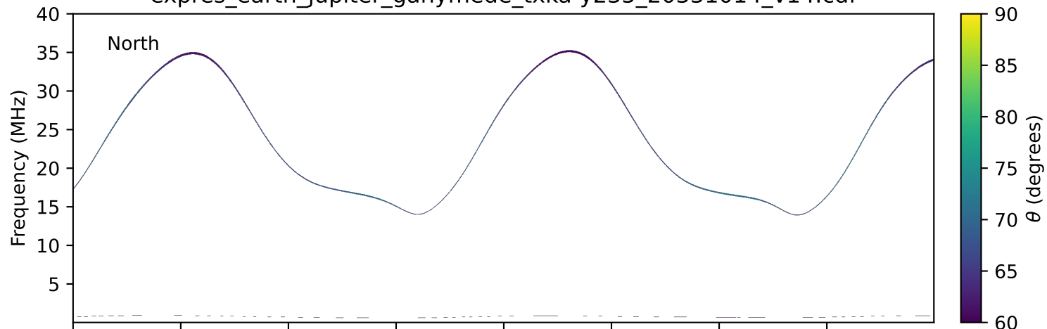
expres_earth_jupiter_ganymede_txka-y235_20331014_v14.cdf
