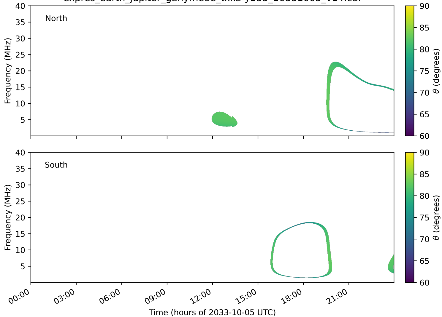
expres_earth_jupiter_ganymede_txka-y235_20331005_v14.cdf
