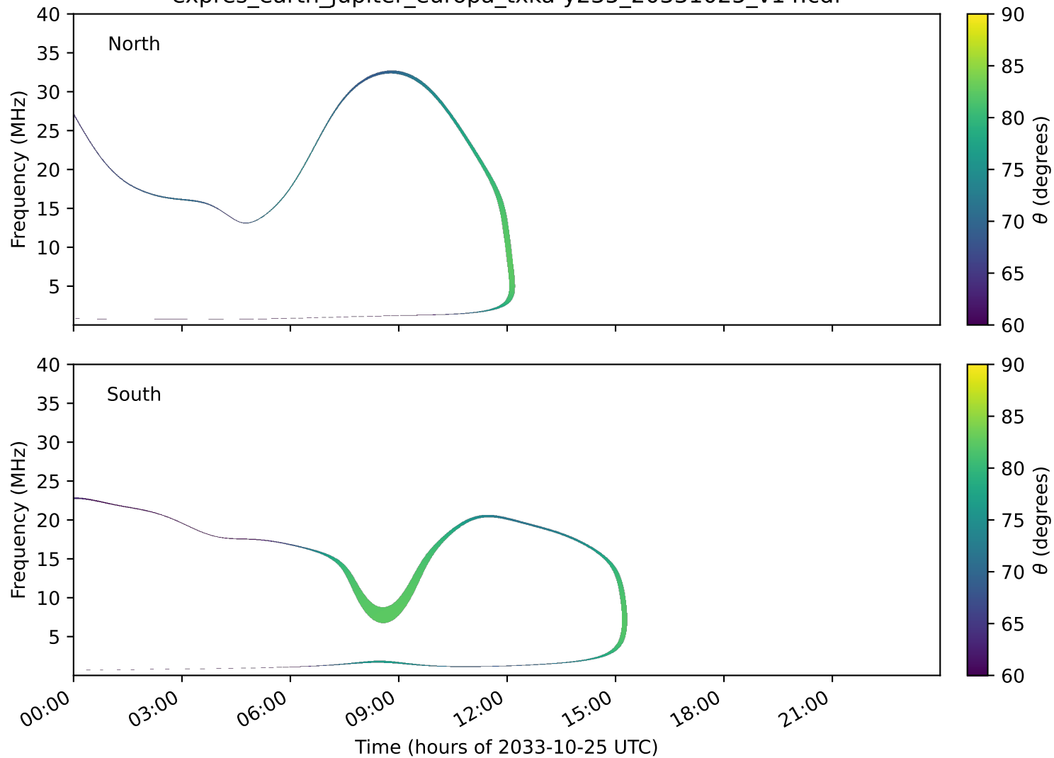
expres_earth_jupiter_europa_txka-y235_20331025_v14.cdf
