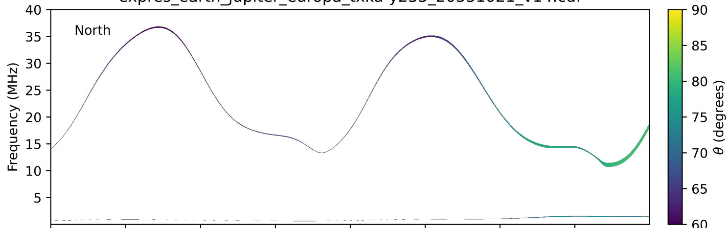
expres_earth_jupiter_europa_txka-y235_20331021_v14.cdf
