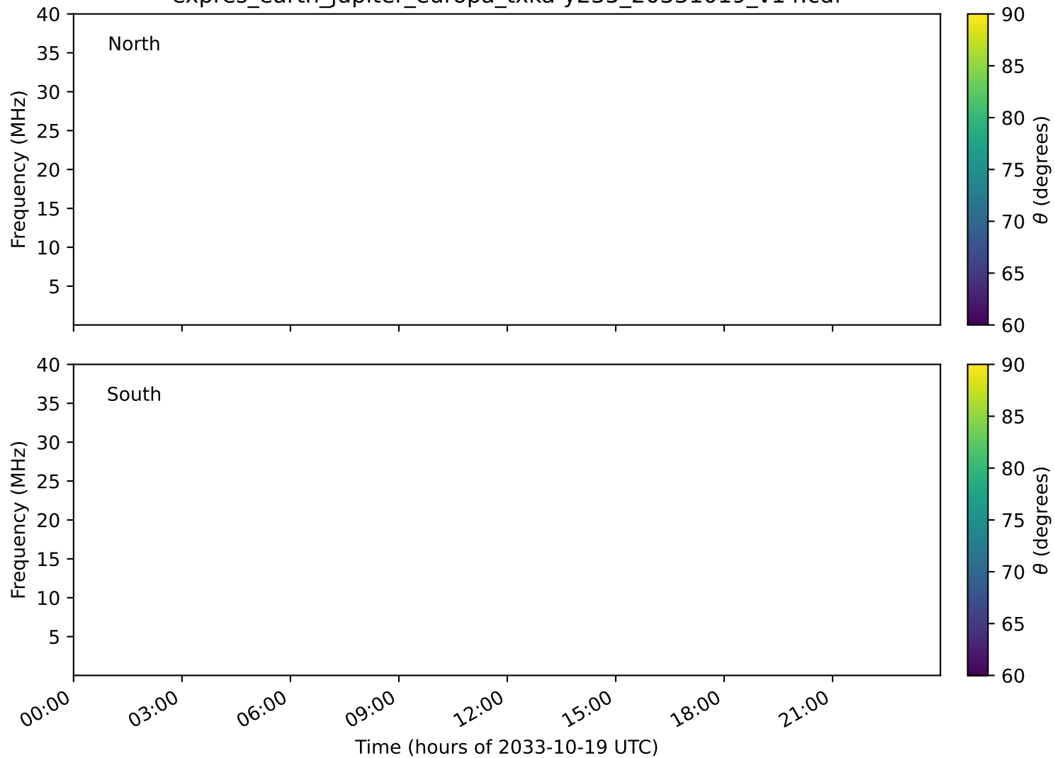
expres_earth_jupiter_europa_txka-y235_20331019_v14.cdf
