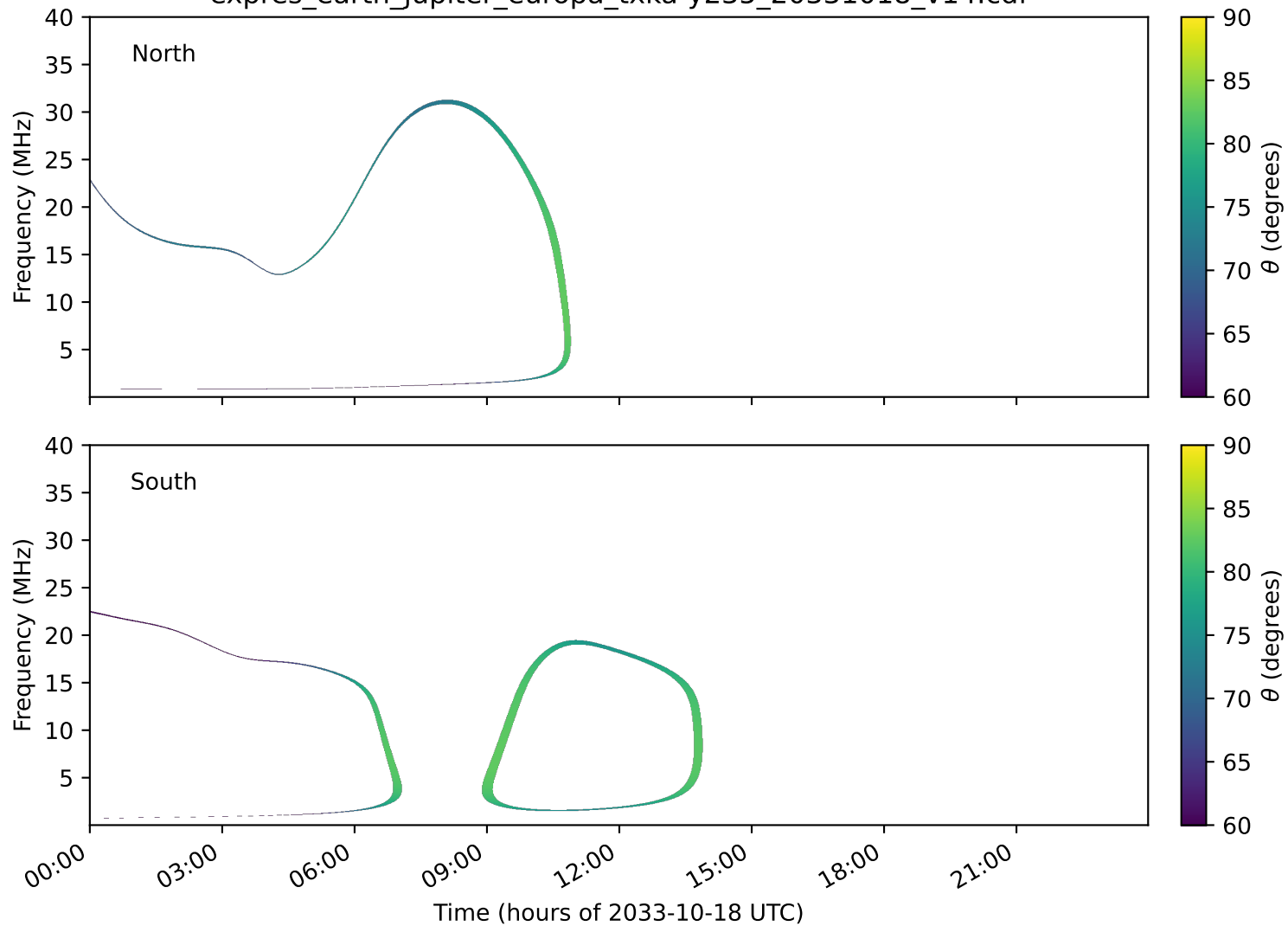
expres_earth_jupiter_europa_txka-y235_20331018_v14.cdf
