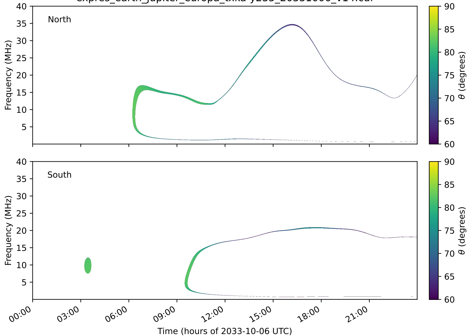
expres_earth_jupiter_europa_txka-y235_20331006_v14.cdf
