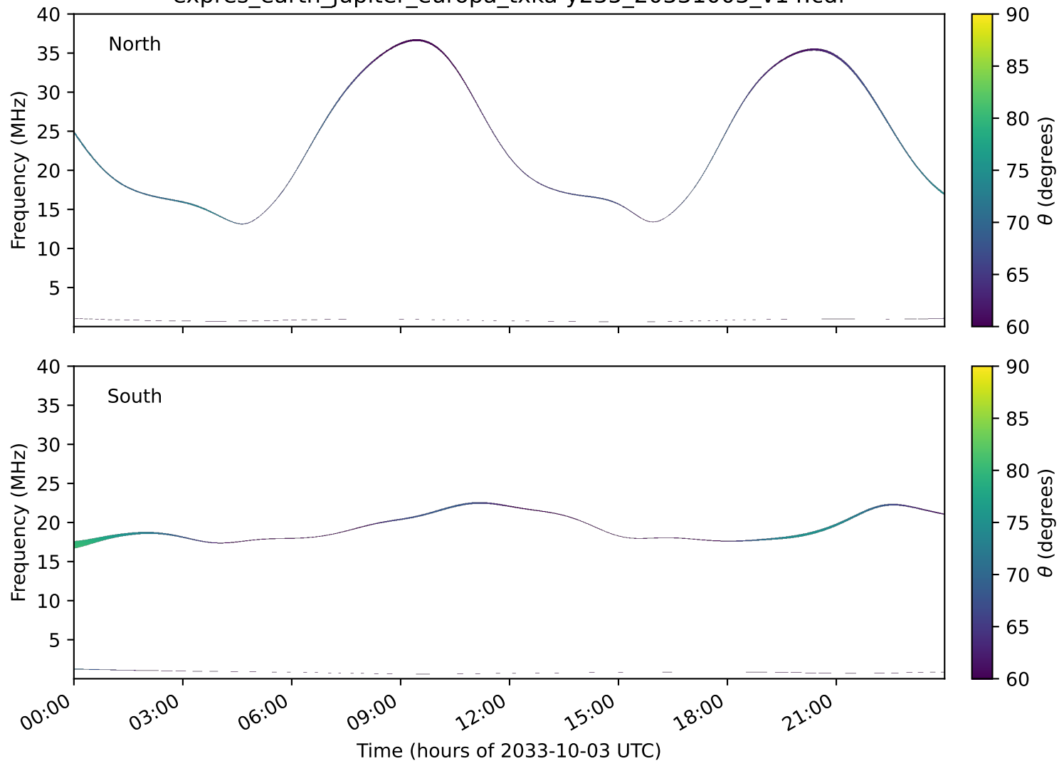
expres_earth_jupiter_europa_txka-y235_20331003_v14.cdf
