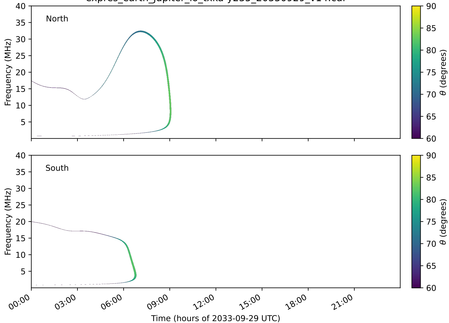
expres_earth_jupiter_io_txka-y235_20330929_v14.cdf
