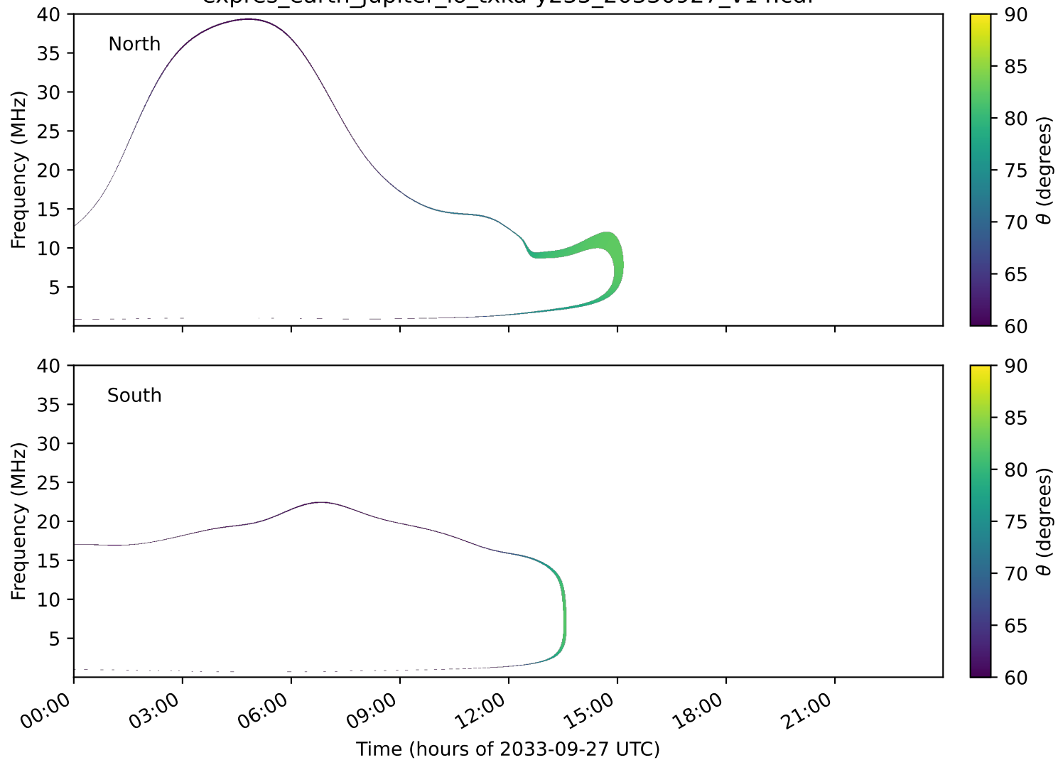
expres_earth_jupiter_io_txka-y235_20330927_v14.cdf
