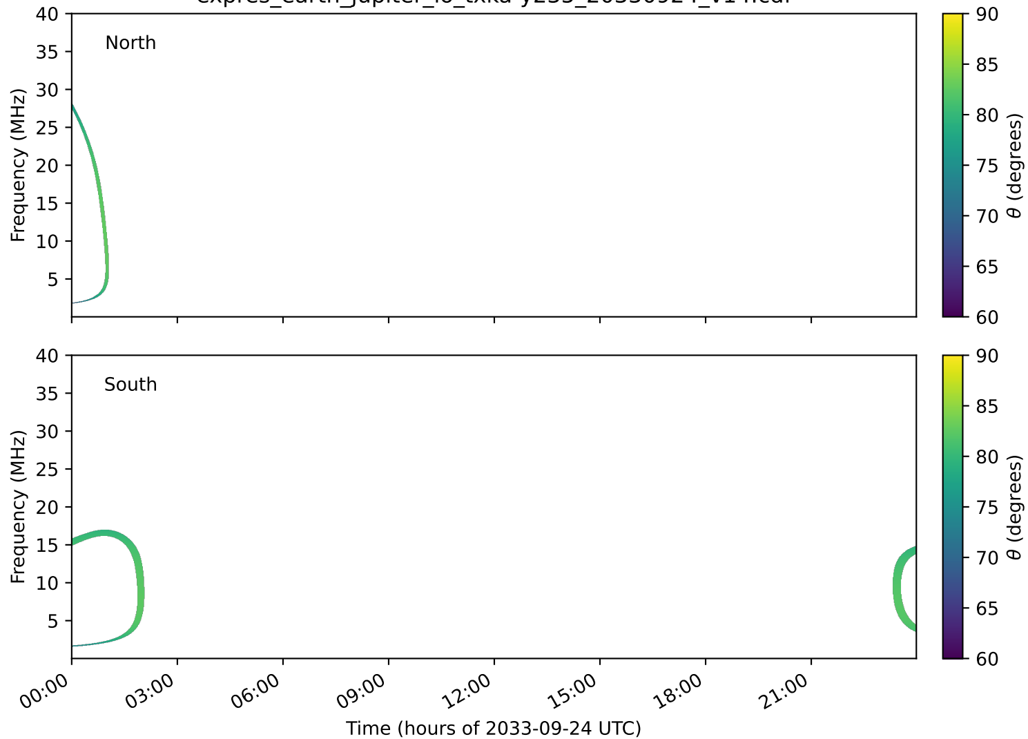
expres_earth_jupiter_io_txka-y235_20330924_v14.cdf
