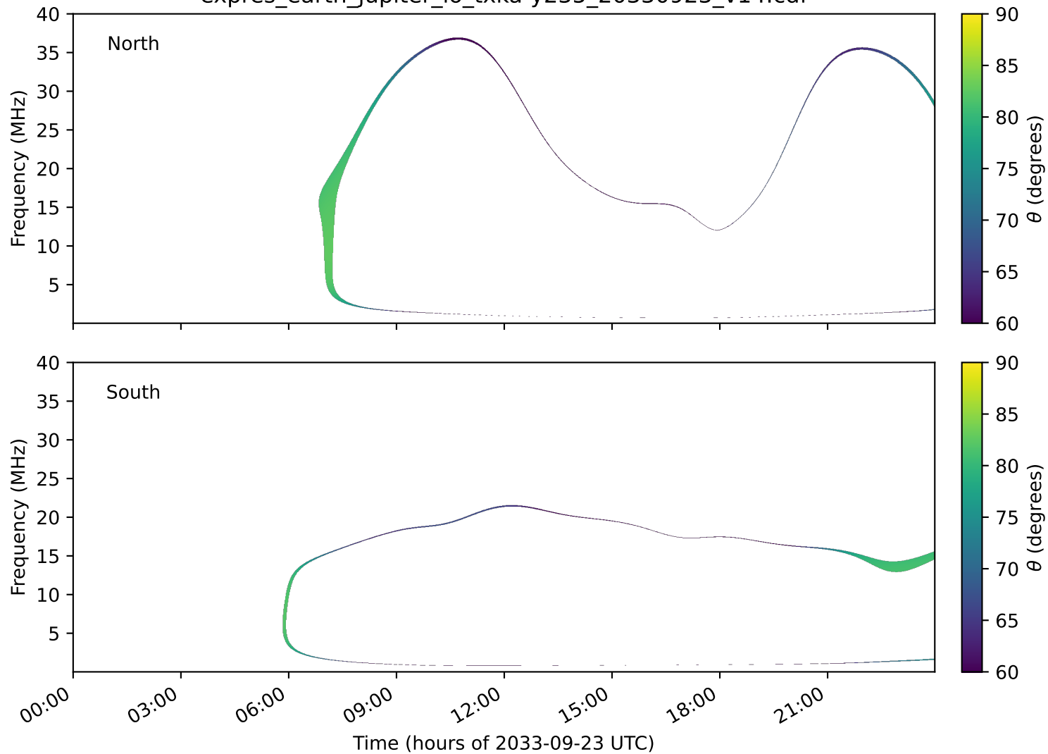
expres_earth_jupiter_io_txka-y235_20330923_v14.cdf
