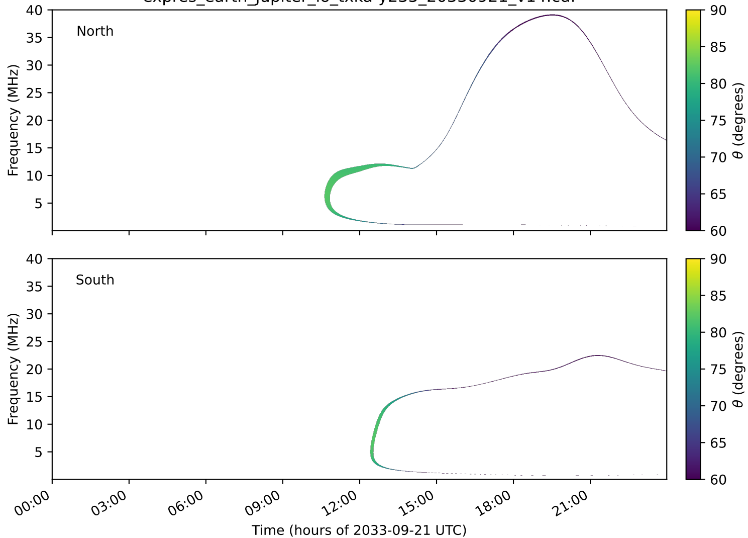
expres_earth_jupiter_io_txka-y235_20330921_v14.cdf
