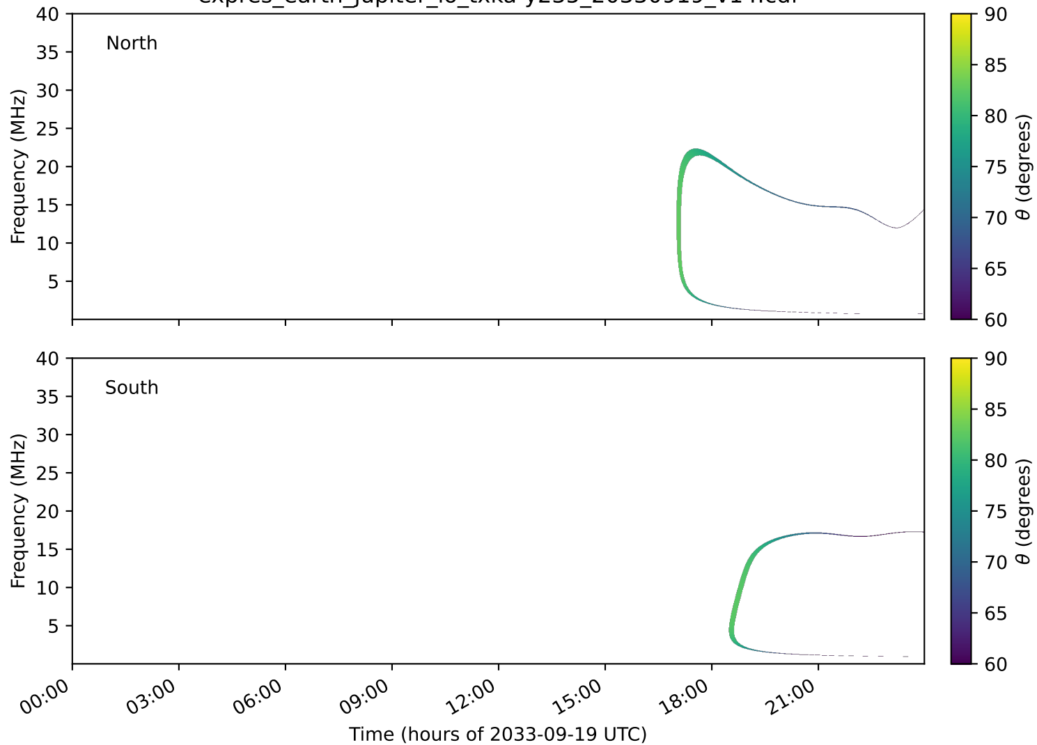
expres_earth_jupiter_io_txka-y235_20330919_v14.cdf
