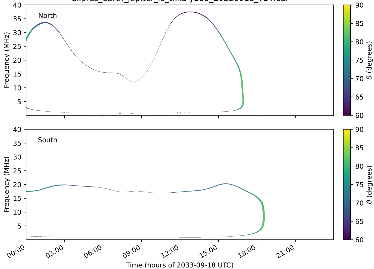
expres_earth_jupiter_io_txka-y235_20330918_v14.cdf
