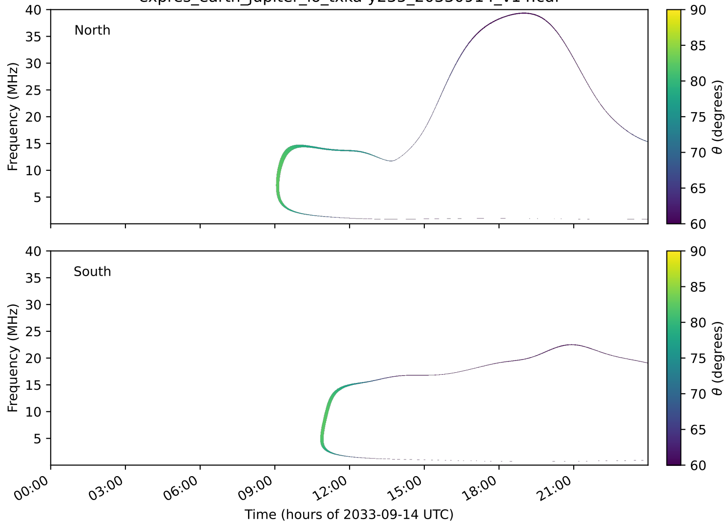
expres_earth_jupiter_io_txka-y235_20330914_v14.cdf
