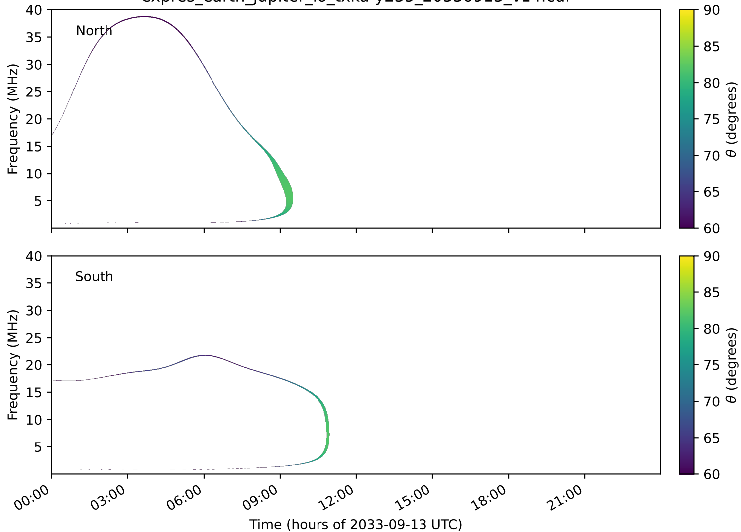
expres_earth_jupiter_io_txka-y235_20330913_v14.cdf
