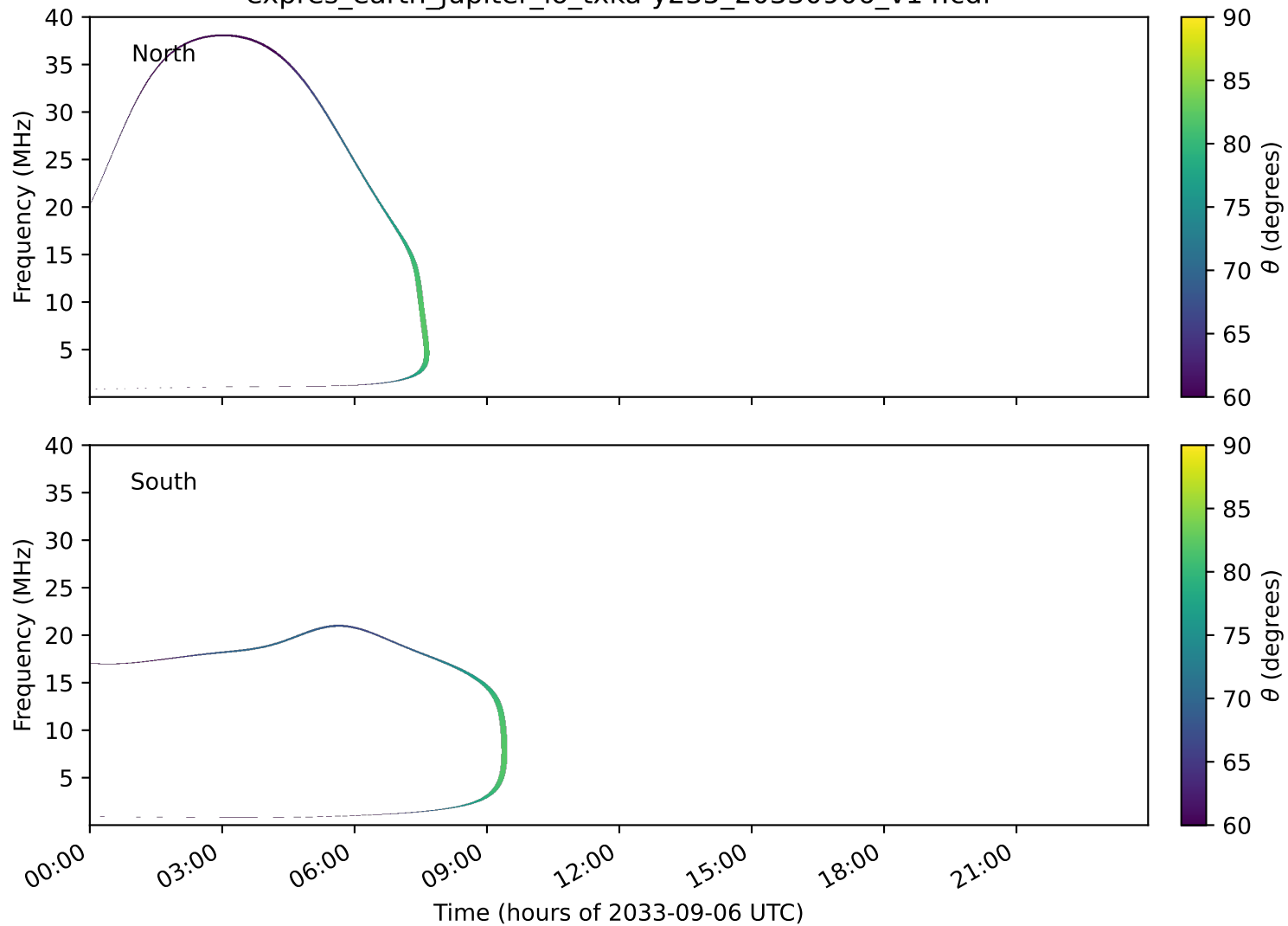
expres_earth_jupiter_io_txka-y235_20330906_v14.cdf
