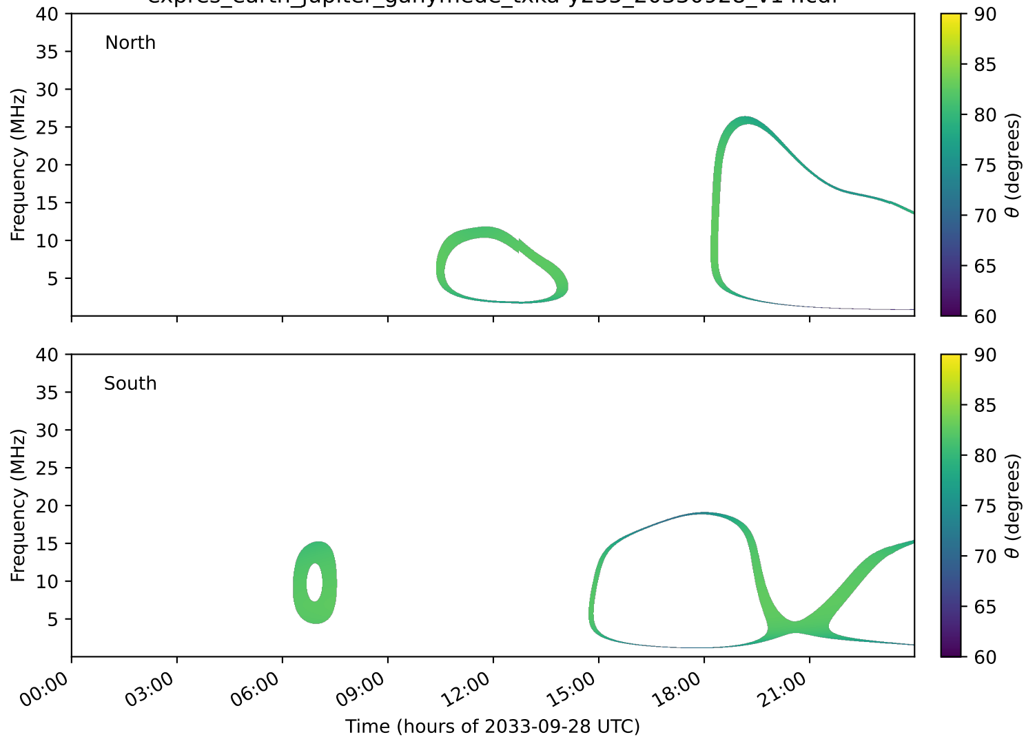
expres_earth_jupiter_ganymede_txka-y235_20330928_v14.cdf
