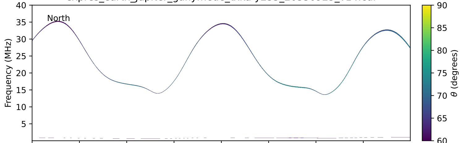
expres_earth_jupiter_ganymede_txka-y235_20330923_v14.cdf
