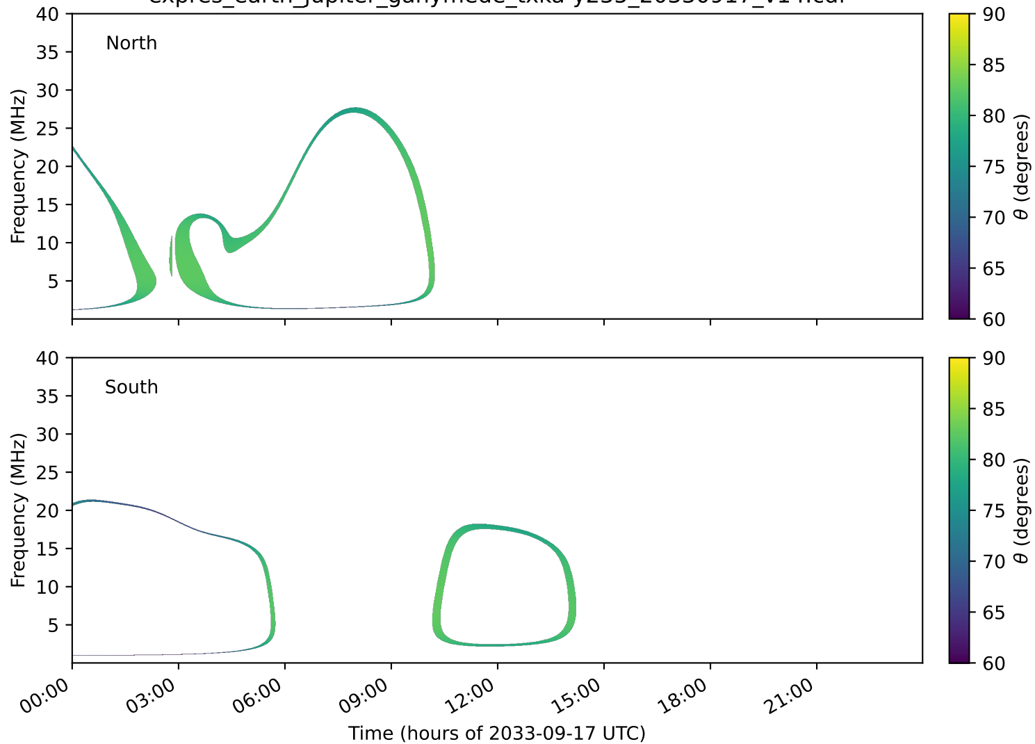
expres_earth_jupiter_ganymede_txka-y235_20330917_v14.cdf
