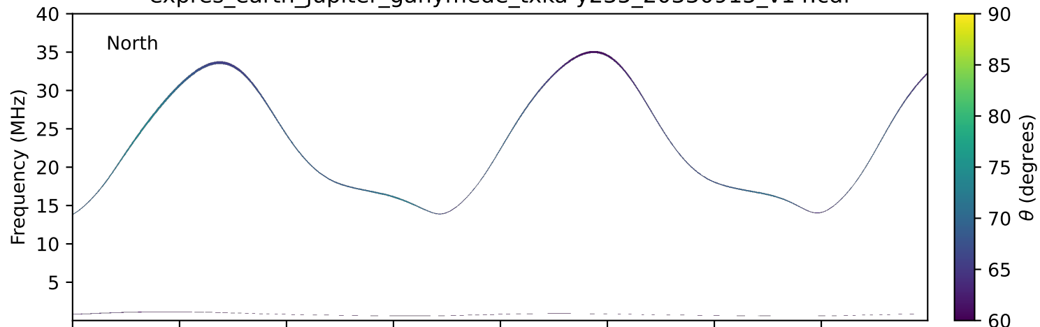
expres_earth_jupiter_ganymede_txka-y235_20330915_v14.cdf
