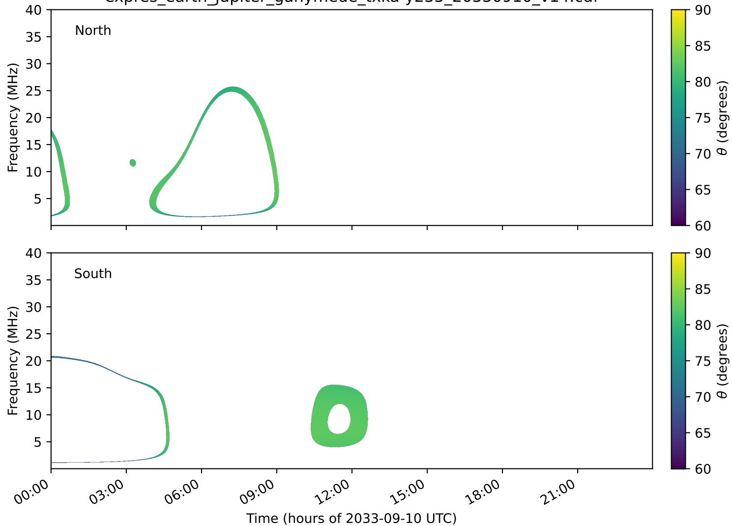
expres_earth_jupiter_ganymede_txka-y235_20330910_v14.cdf
