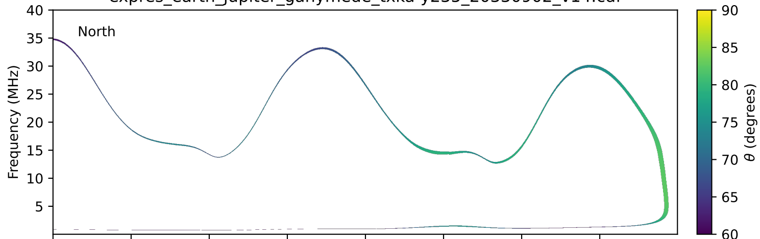
expres_earth_jupiter_ganymede_txka-y235_20330902_v14.cdf
