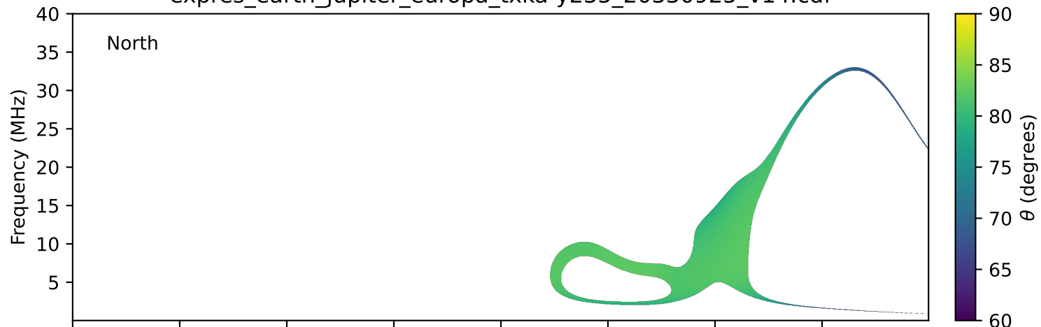
expres_earth_jupiter_europa_txka-y235_20330925_v14.cdf
