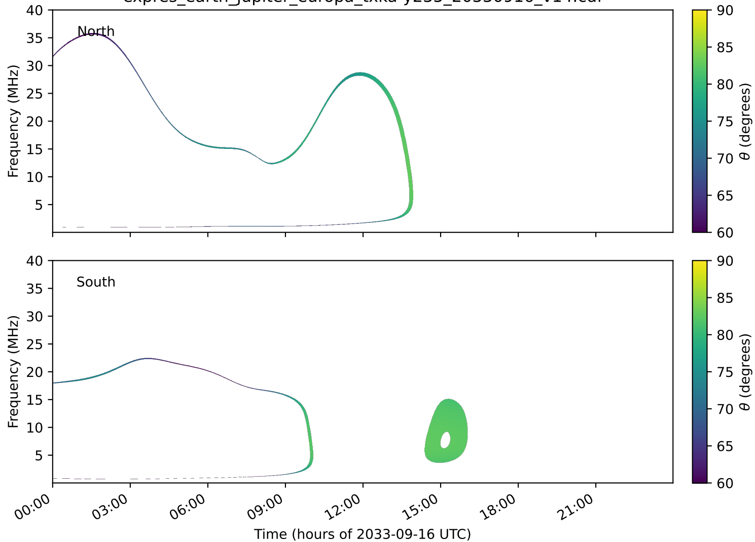
expres_earth_jupiter_europa_txka-y235_20330916_v14.cdf
