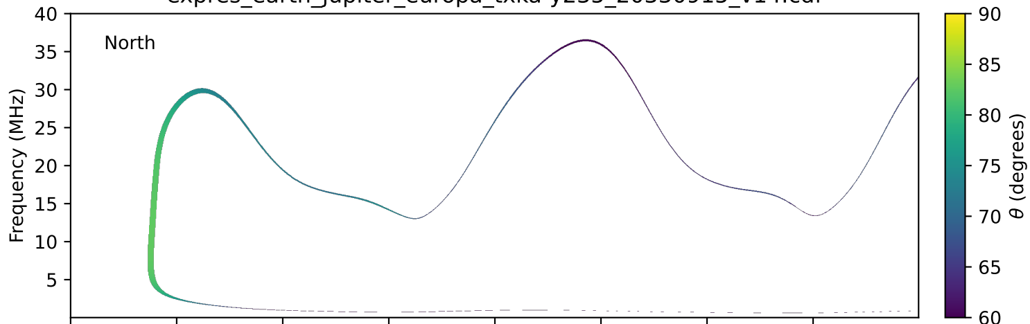
expres_earth_jupiter_europa_txka-y235_20330915_v14.cdf
