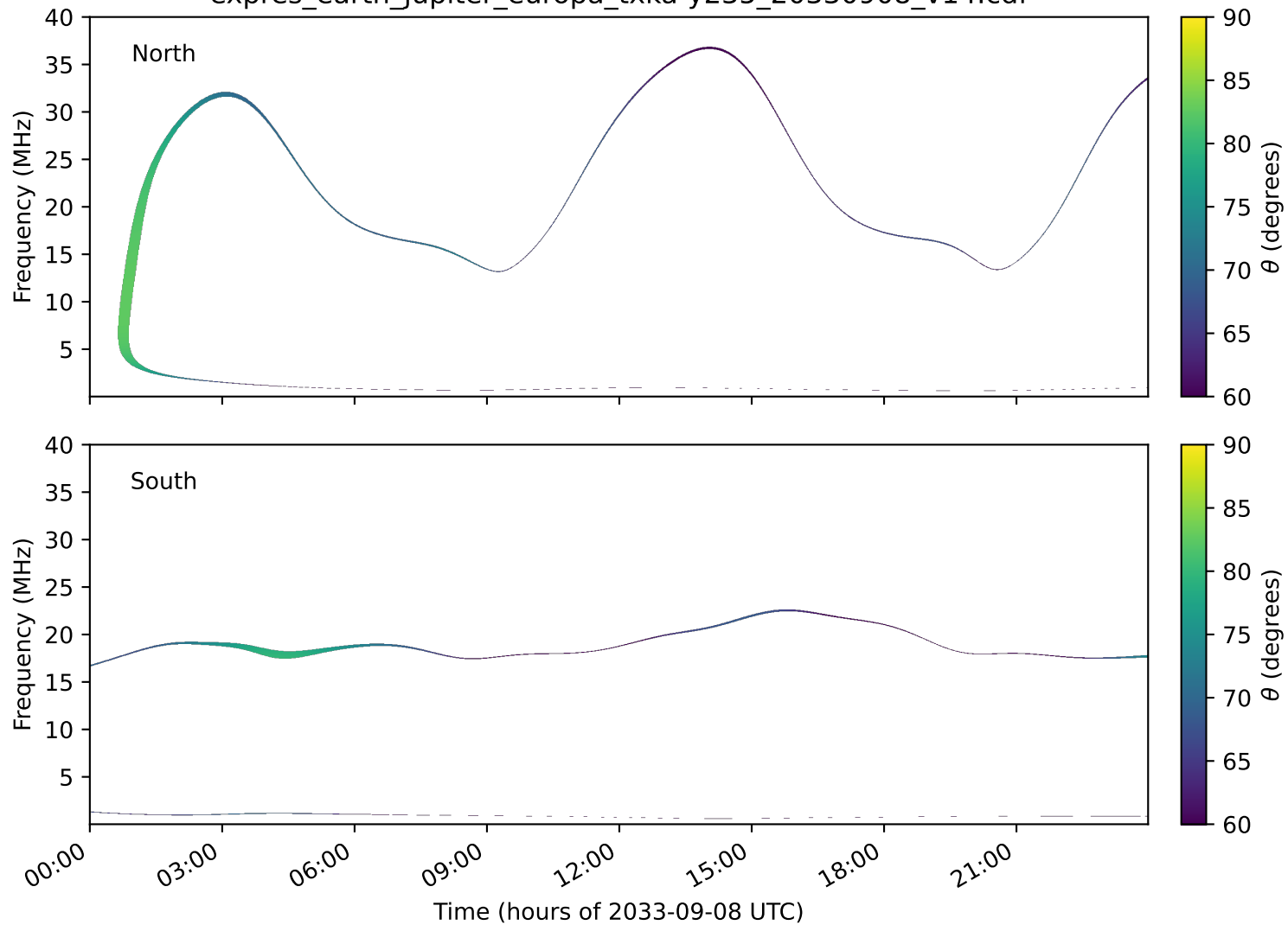
expres_earth_jupiter_europa_txka-y235_20330908_v14.cdf
