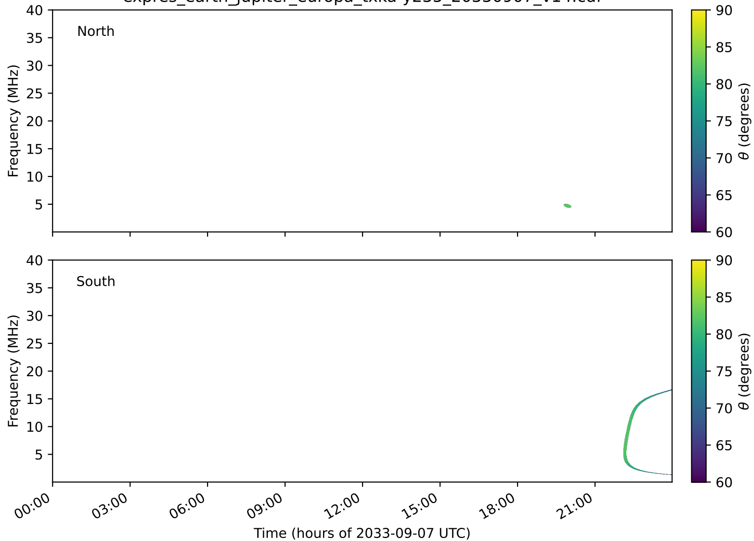
expres_earth_jupiter_europa_txka-y235_20330907_v14.cdf
