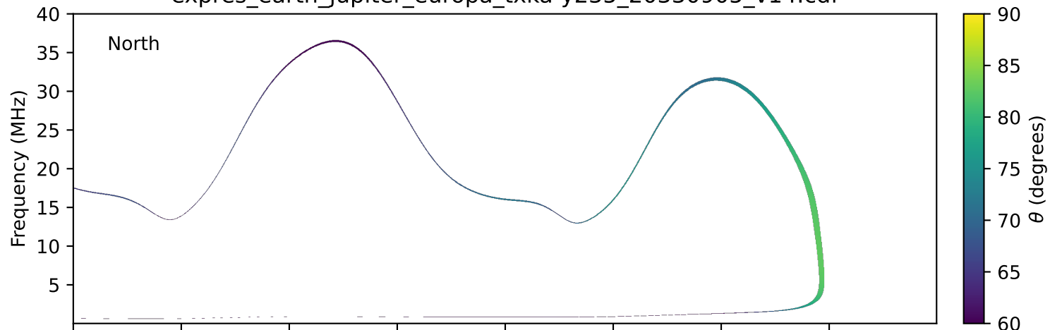
expres_earth_jupiter_europa_txka-y235_20330905_v14.cdf
