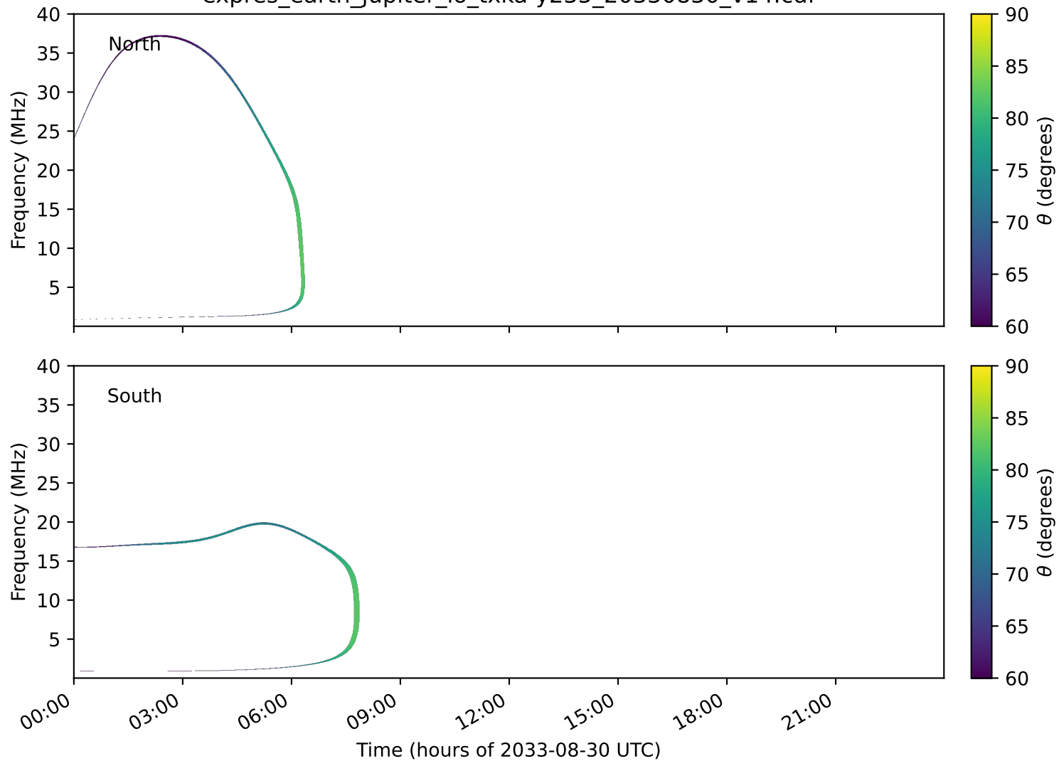
expres_earth_jupiter_io_txka-y235_20330830_v14.cdf
