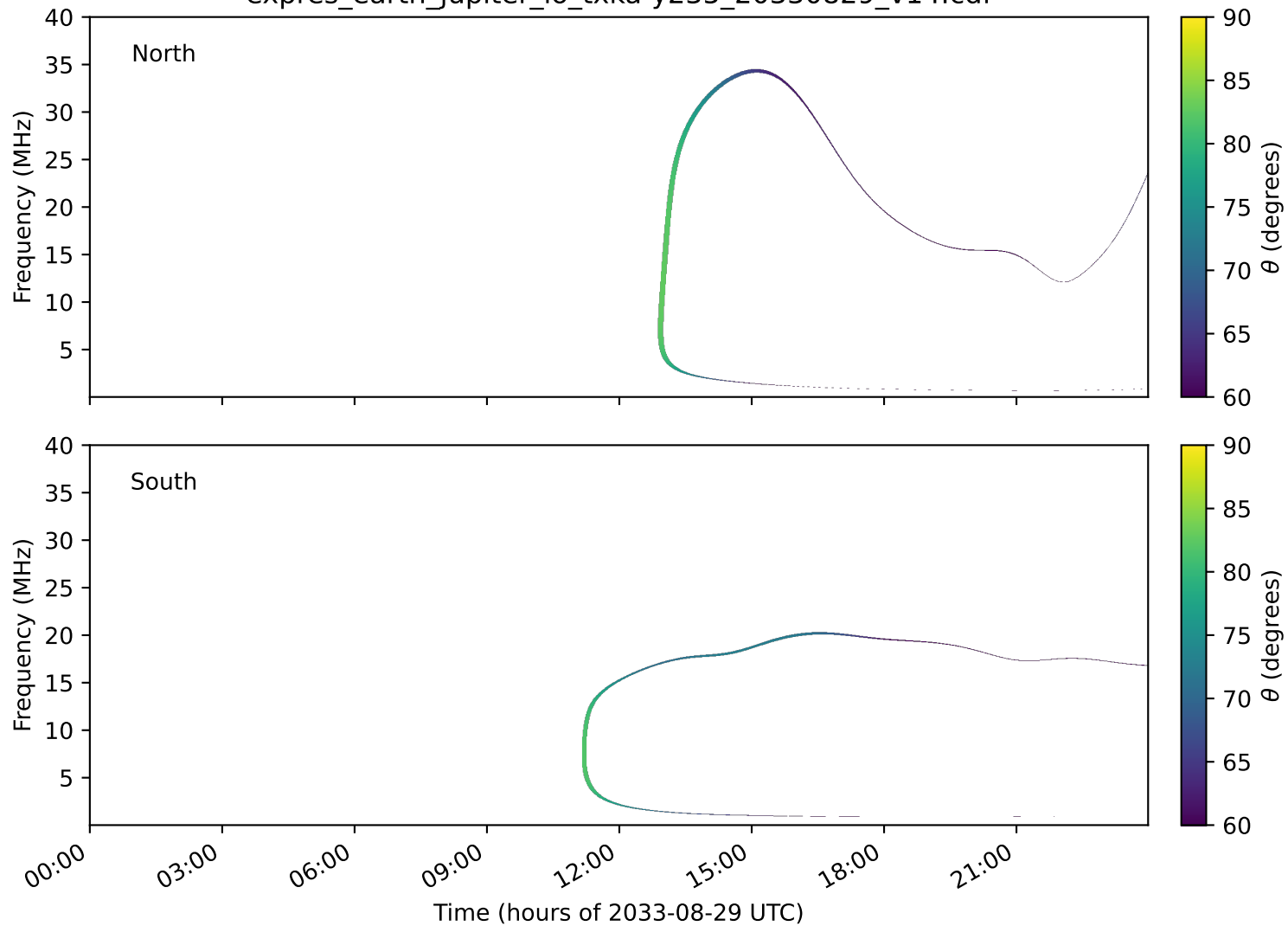
expres_earth_jupiter_io_txka-y235_20330829_v14.cdf
