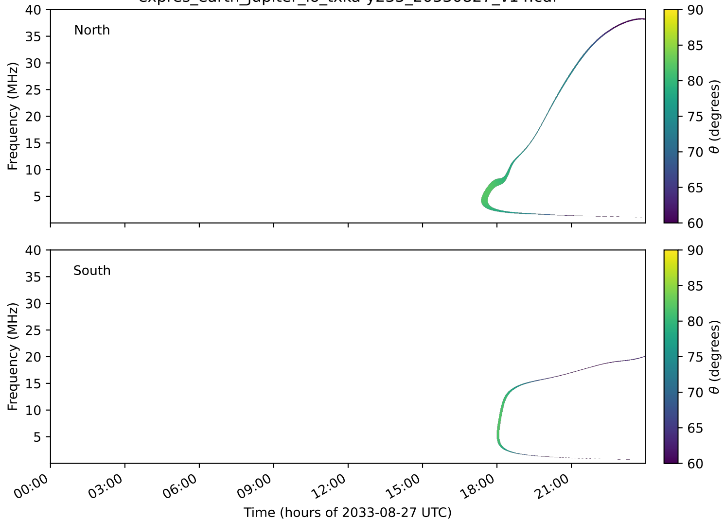
expres_earth_jupiter_io_txka-y235_20330827_v14.cdf
