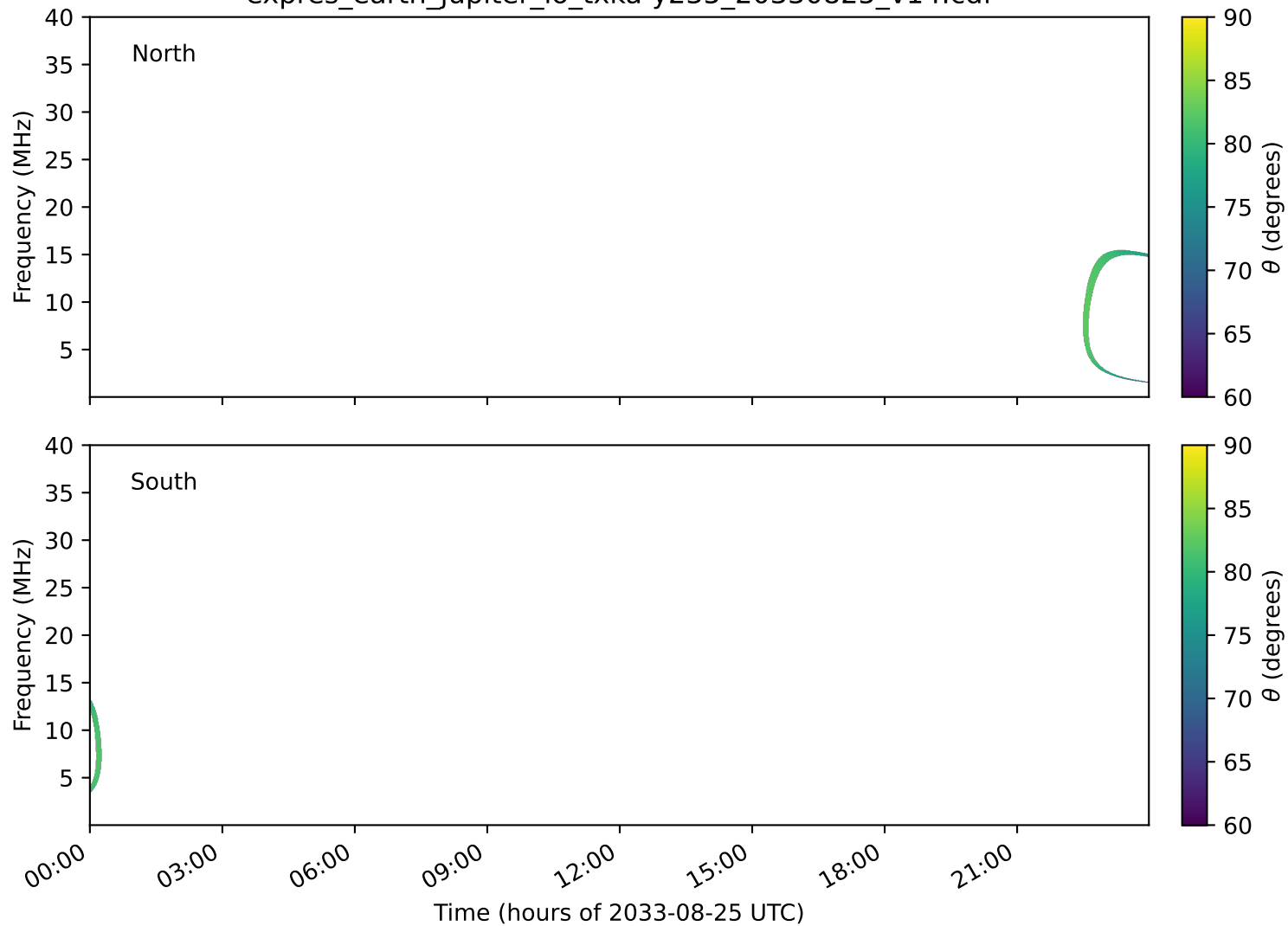
expres_earth_jupiter_io_txka-y235_20330825_v14.cdf
