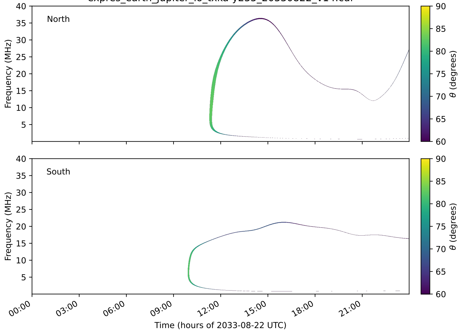
expres_earth_jupiter_io_txka-y235_20330822_v14.cdf
