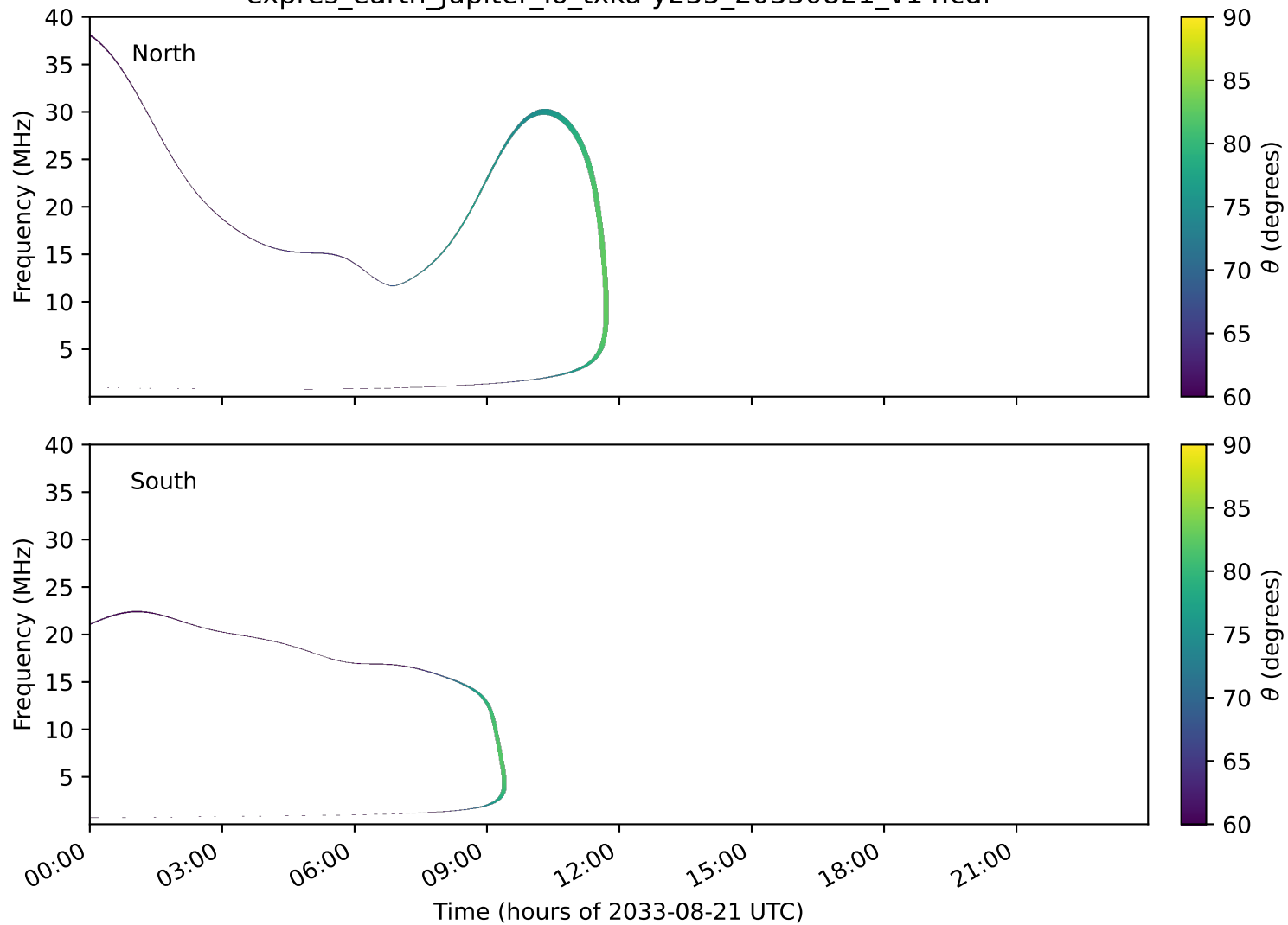
expres_earth_jupiter_io_txka-y235_20330821_v14.cdf
