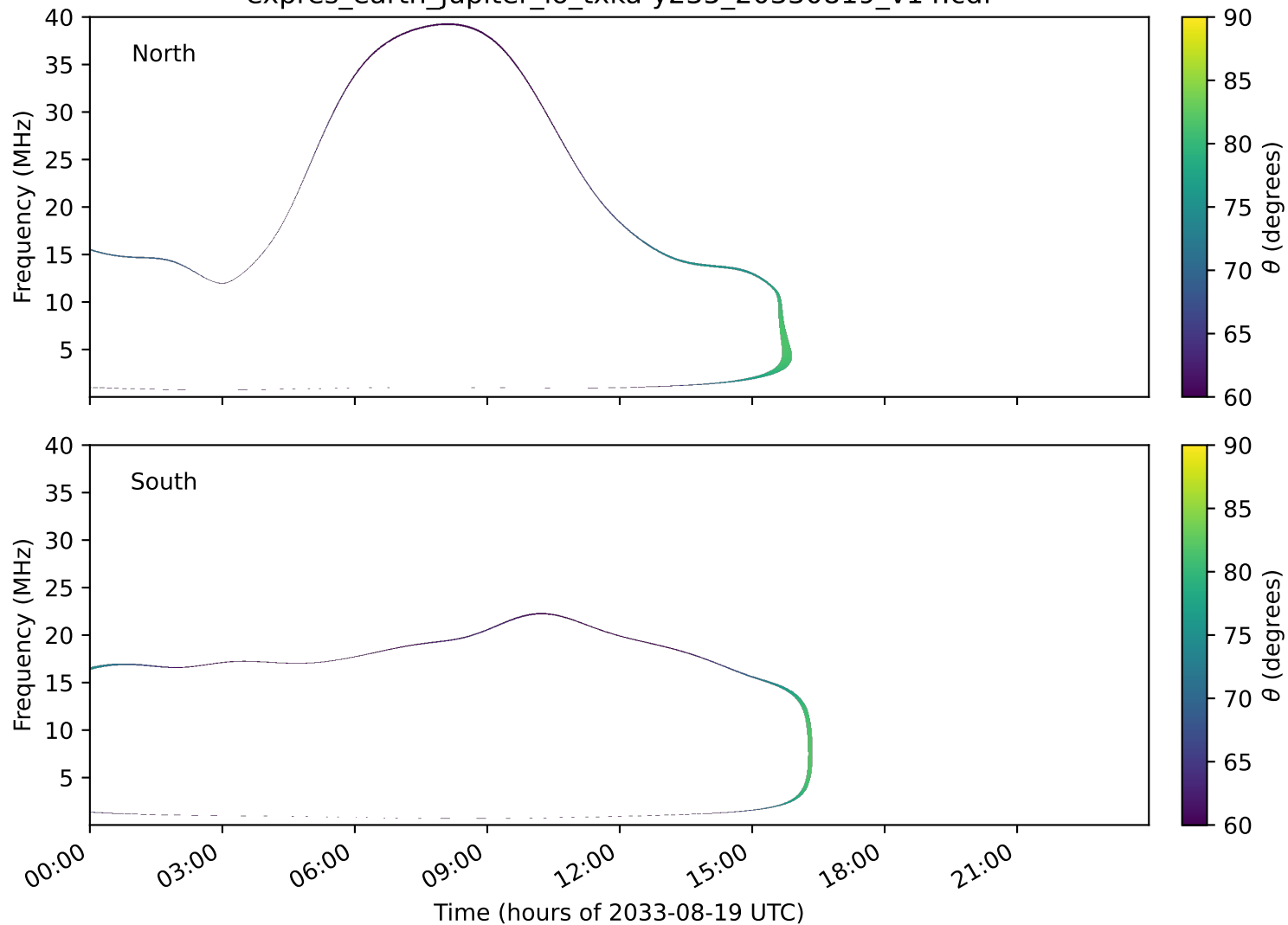
expres_earth_jupiter_io_txka-y235_20330819_v14.cdf
