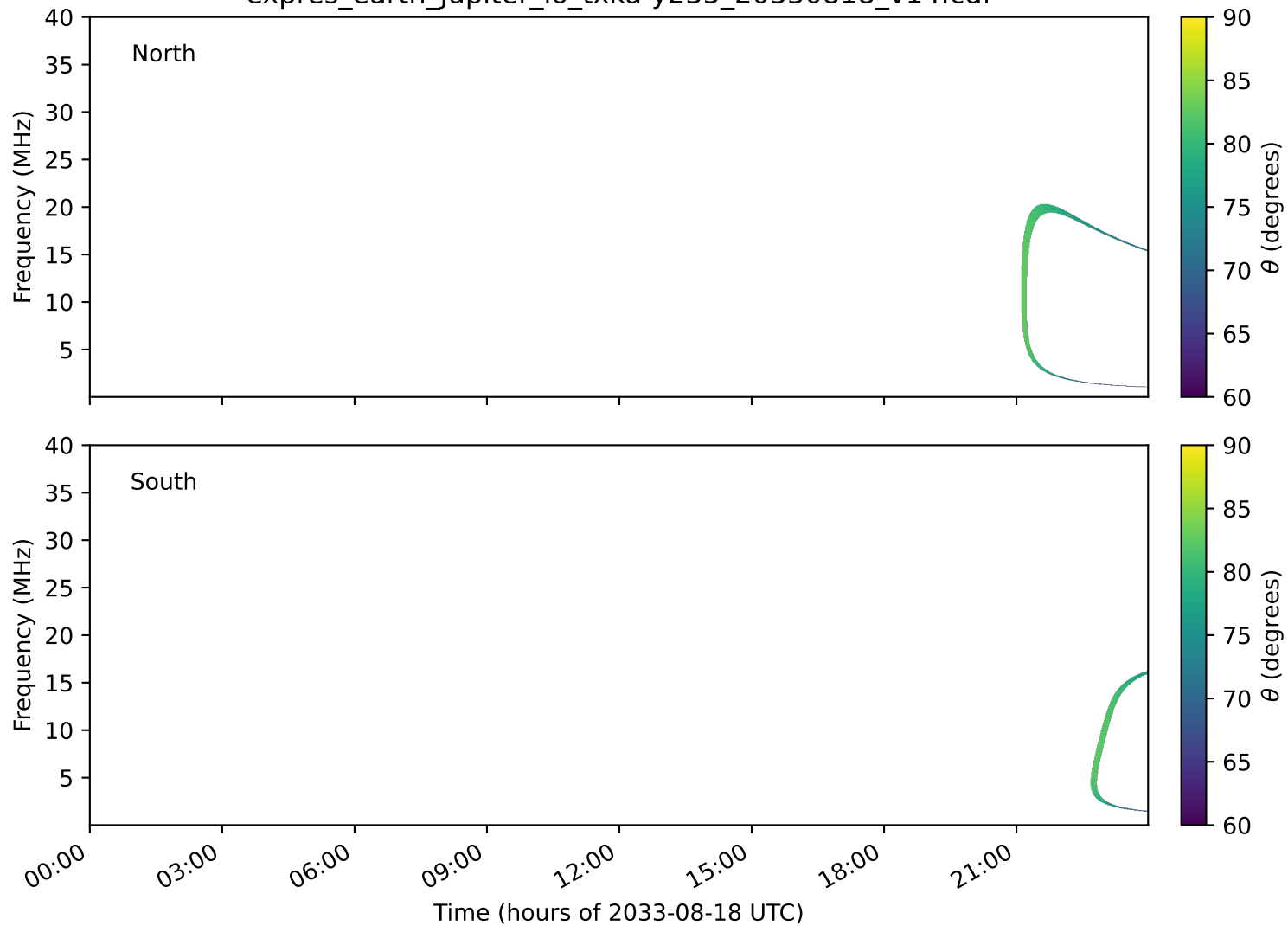
expres_earth_jupiter_io_txka-y235_20330818_v14.cdf
