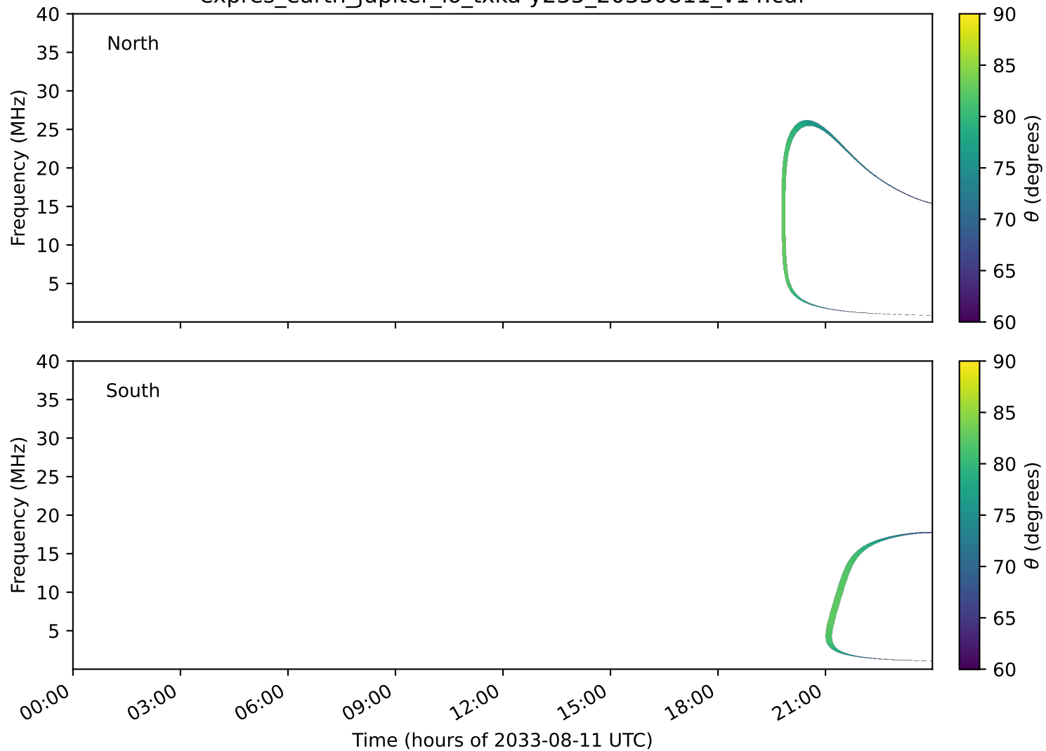
expres_earth_jupiter_io_txka-y235_20330811_v14.cdf
